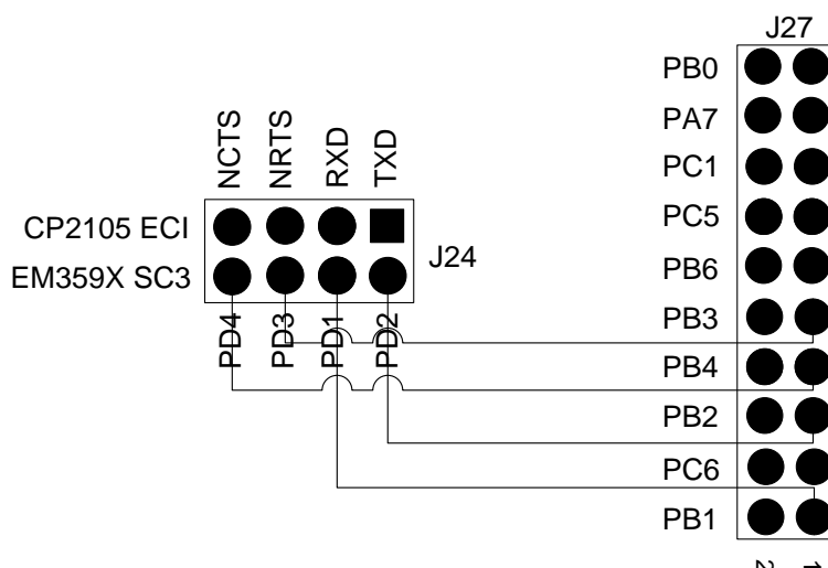
Figure 4. Jumper Wire Settings Required for EM359x SC3 UART Access by Debug Adapter
